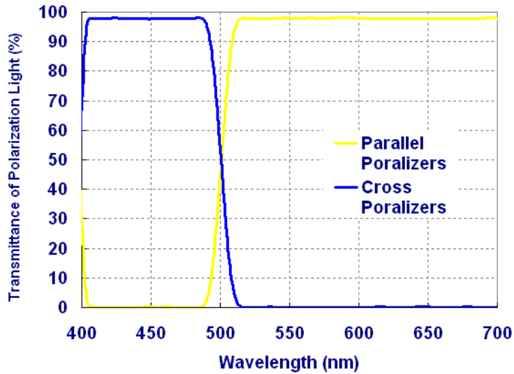
BY Filter
