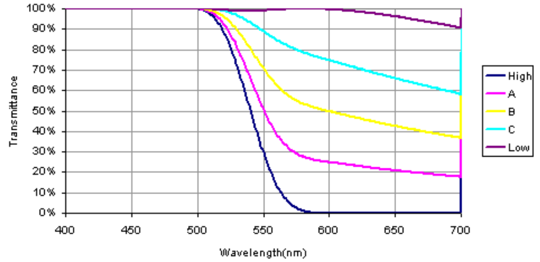
Simulation data
