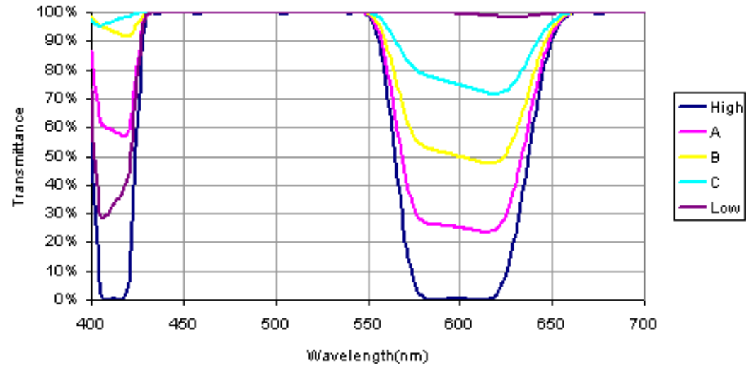
Simulation data
